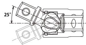
Universal Joint
