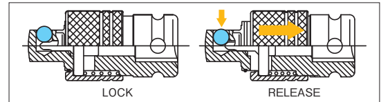
Lock & Quick Release
